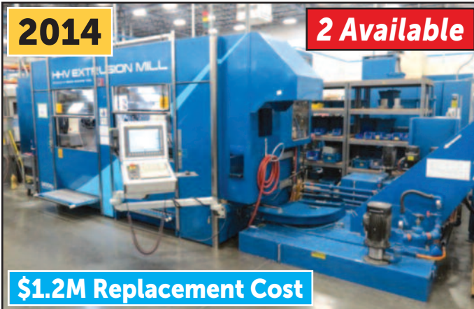
Modig HHV 4-Axis High Speed Extrusion Machining Center
