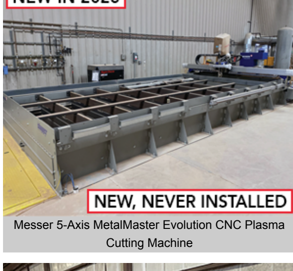
Messer 5-Axis MetalMaster Evolution CNC Plasma Cutting Machine
