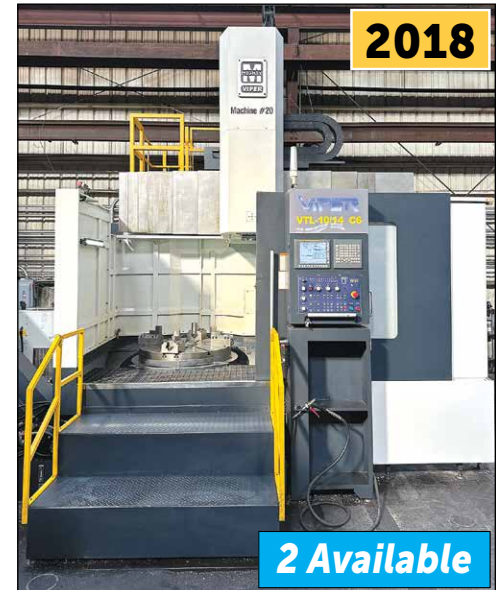
36" Might Viper VTL-10/14 CNC Vertical Boring Mill
